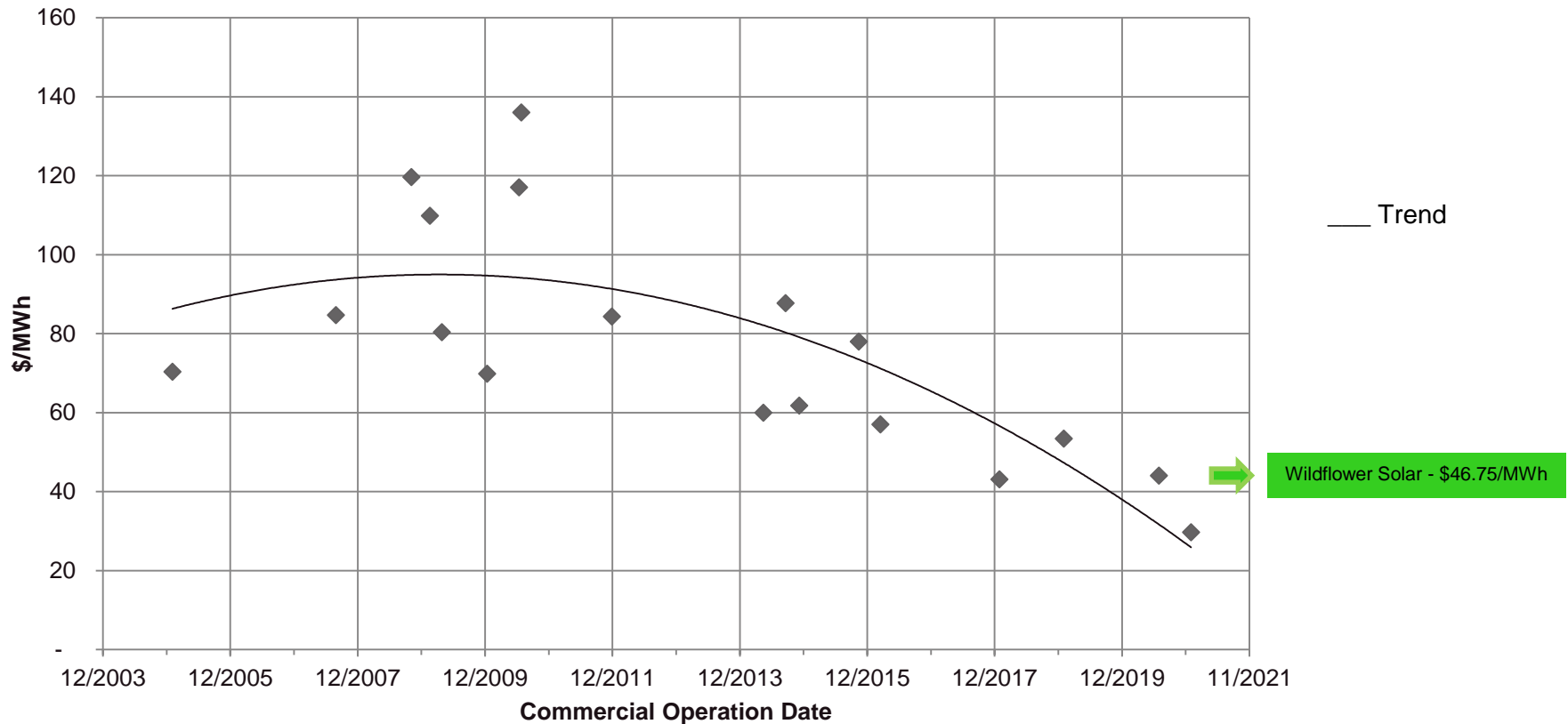
2021 Levelized Cost of Energy ($/MWh) Current SMUD Renewable Power Purchase Agreements
